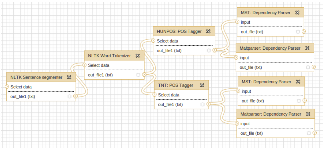
Figure 2: A user-defined LAP workflow with four endpoints. The data processing starts with unannotated text and ends with four datasets containing different annotations.
